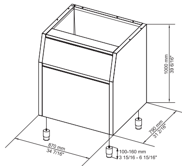
Adjustable feet 3 15/16" – 6 15/16"
